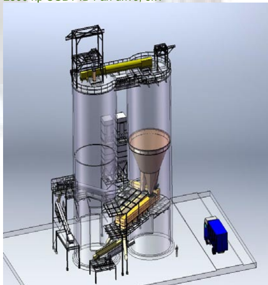
Petcoke /Coal storage and blending 2000Mt
